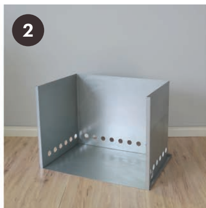
2 Screw inner left, inner right and inner back panels together, returns facing outwards.
